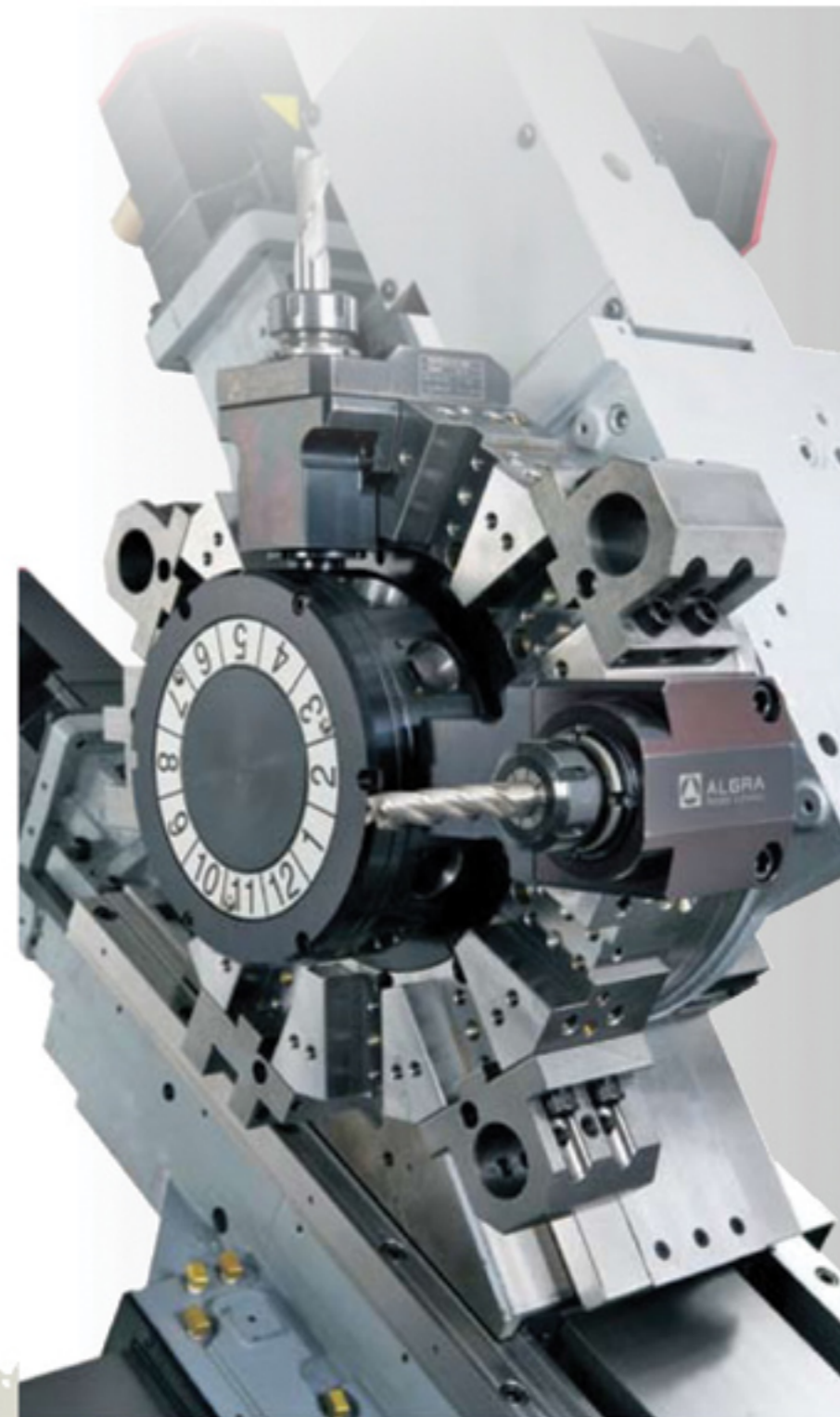
Dodecagonal Power turret
